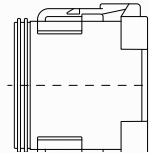
40.56mm W x 18.19mm H x 30.94mm L DT06-12S
